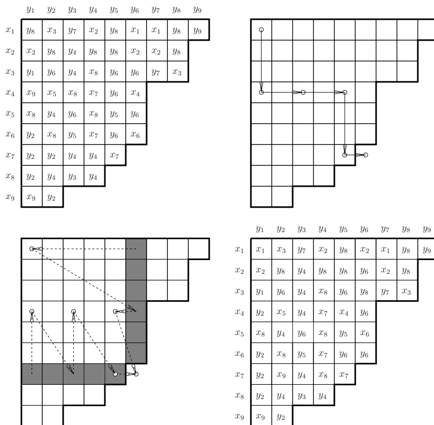
Fig. 2: An example of an arrangement corresponding to the left-hand side of CWBR for \lambda = 988666542 ; hook walk; shift of labels; final arrangement.
