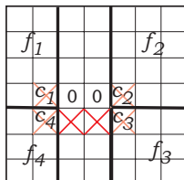
Fig. 3: A polyomino of area min + 1 constructed from a bench polyomino
