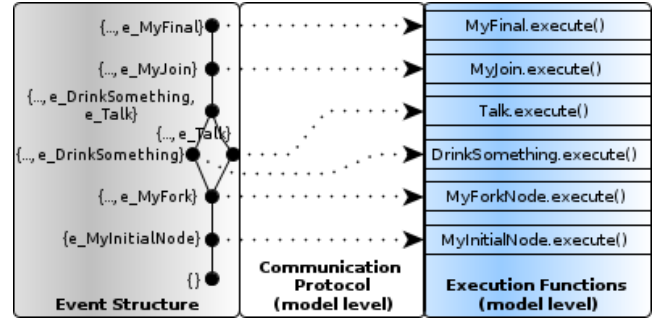
Figure 3. Application of the separation of concerns to the example from Figure 1.
