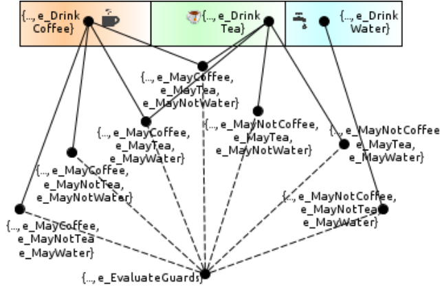
Figure 11. Close-up on the DecisionNode part of the simplified Event Structure of the example model
