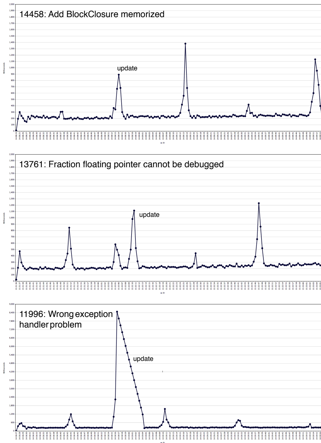
Figure 4. Response Time Graph of SmalltalkHub Application. Running an application during 90 seconds with an update at second 30. Simple updates create pauses similar to garbage collections. After the update the application returns to its usual performance level.
