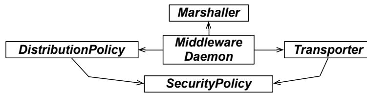
Figure 9 – Core classes of our adaptable middleware
