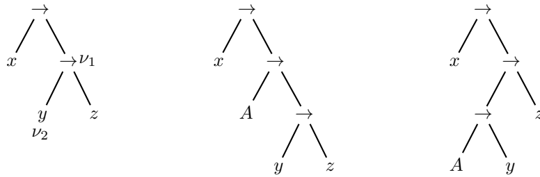
Fig. 2: The left tree is T , the other trees are the (\nu_1, A) -expansion and (\nu_2, A) -expansion of T .
