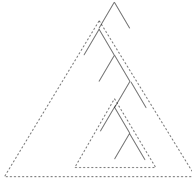
Fig. 3: The left subtrees \Delta_\nu and \Delta_\nu^2 associated to a node \nu of a tree.
