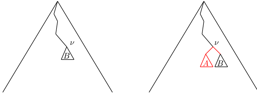
Fig. 1: The right tree is the (\nu, A) -expansion of the left one.
