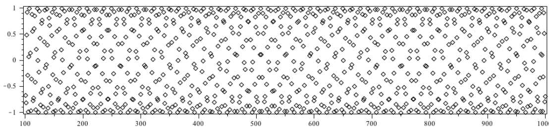
Fig. 3: Maple plot of -\frac{\sqrt{n} R^{n+1/2} a_n}{2\sqrt{\pi}} for 100 \leq n \leq 1000 .
