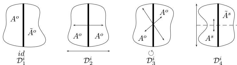
Fig. 5: Decomposition of inner edge rooted dissections
