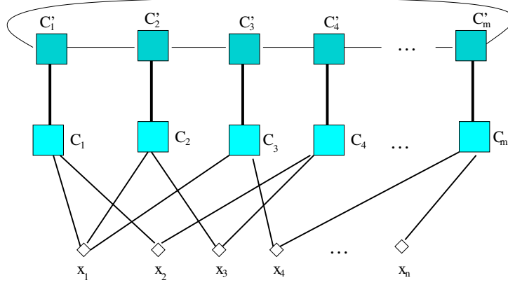
Fig. 1: Figure 4.1: The underlying graph of a bounded-degree monotone linear threshold Boolean S(y)DS in the construction of Theorem 4.2. The original clause nodes are marked C_j , the cloned clause nodes are primed, as in C'_j , and the variable nodes are denoted by x_i .
