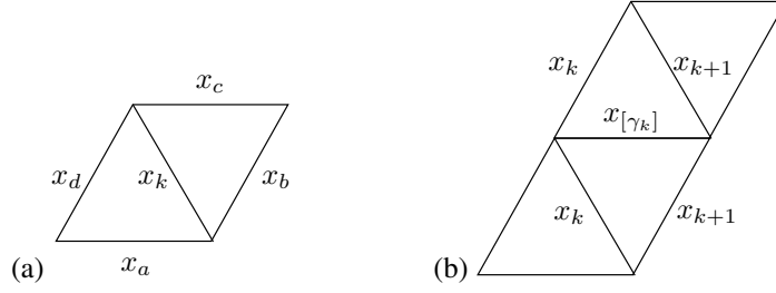
Fig. 1: (a) The tile \bar{S}_k ; (b) Glueing tiles S_k and S_{k+1} along the edge weighted x_{[\gamma_k]}
