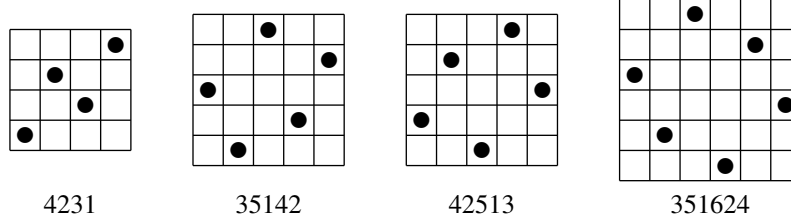
Fig. 3: The four forbidden patterns.
