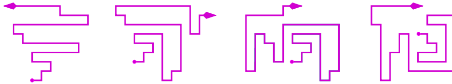
Fig. 2: Four prudent walks: the first one is 1-sided, the others are respectively 2-sided, 3-sided and 4-sided.
