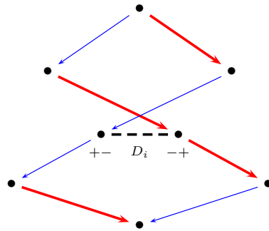
Fig. 5: Constructing \mathcal{G}(\mathcal{X}) from \mathcal{X} ; here we have F_{i-1} \swarrow, F_i \searrow .
