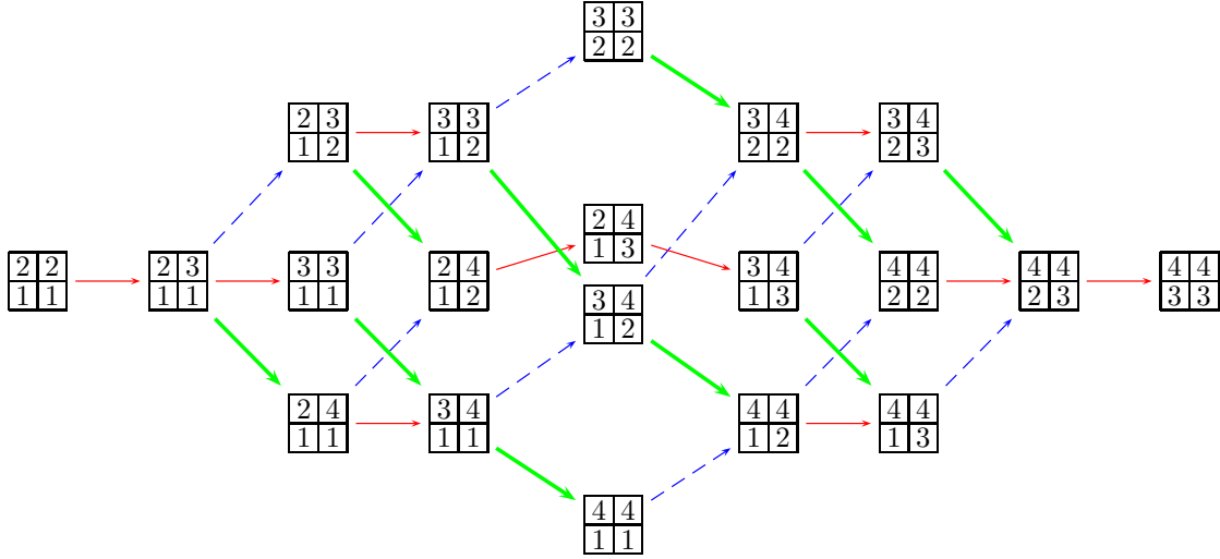
Fig. 1: The crystal graph \mathcal{X}_{(2,2)}^4 , with edges \tilde{f}_1 \nearrow , \tilde{f}_2 \rightarrow , \tilde{f}_3 \searrow .
