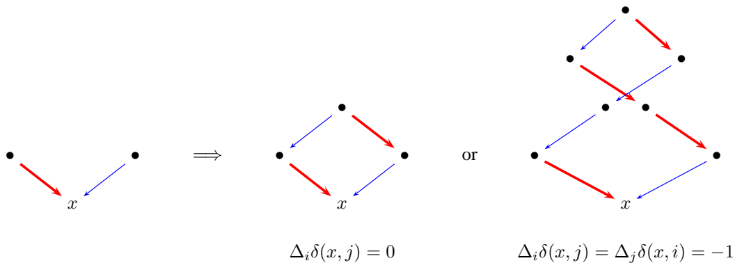
Fig. 3: An illustration of axioms P5 and P6, where F_j \swarrow, F_i \searrow .
