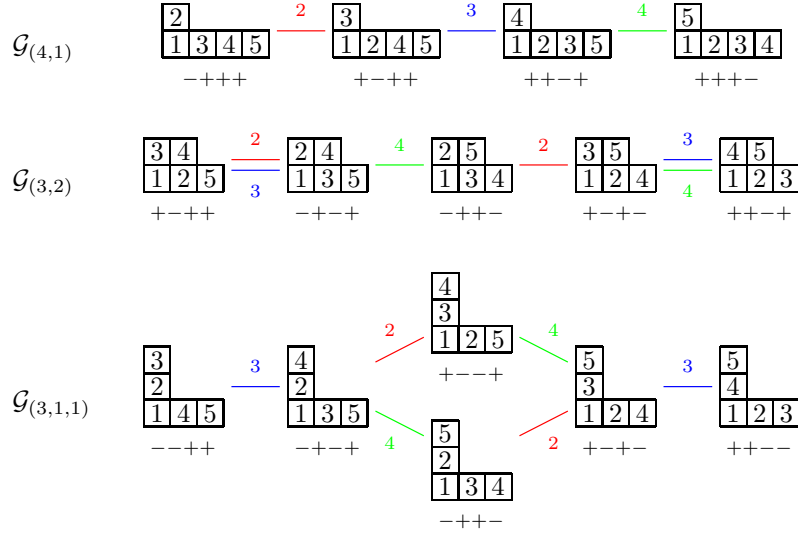
Fig. 4: The standard dual equivalence graphs \mathcal{G}_{(4,1)} , \mathcal{G}_{(3,2)} and \mathcal{G}_{(3,1,1)} .
