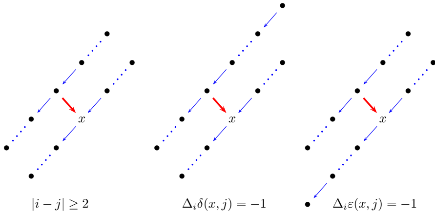
Fig. 2: An illustration of axioms P3 and P4, where F_j \swarrow, F_i \searrow .
