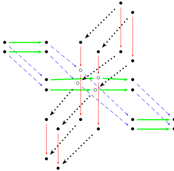
Fig. 6: An illustration of the commutativity which establishes dual equivalence axiom 4; the 0-weight vertices are o's and crystal operators are F_{i-3} \searrow , F_{i-2} \rightarrow , F_{i-1} \swarrow , F_i \downarrow .
