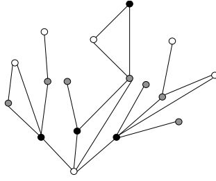
Fig. 2: Example of a Cactus-Tree
