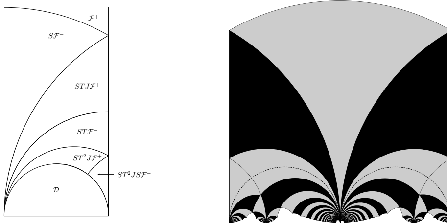
Figure 6: On the left, the six domains which constitute the domain \tilde{\mathcal{B}}_+ \setminus \mathcal{D}_+ . On the right, the disk \mathcal{D} is not compatible with the geometry of transforms of the fundamental domains \mathcal{F} .
