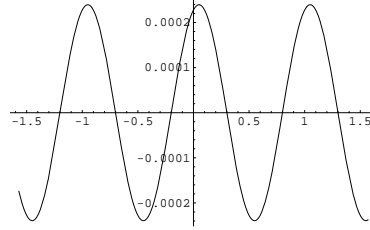
Fig. 3: Plot of the function \phi in the case a = 3 .
