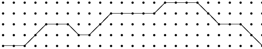
Fig. 2: A Motzkin path with MinPlateau = 2, MaxPlateau = 3, MinLevel = 1 and MaxLevel = 4.
