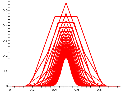
Figure 3: The histograms of the probability distribution \mathbb{P}(A_n = k) as a function of k/(n+1) , for the adverse-campaign urn initialized with (1, 0) and for n = 3 \dots 50 , illustrate convergence to a Gaussian regime.
