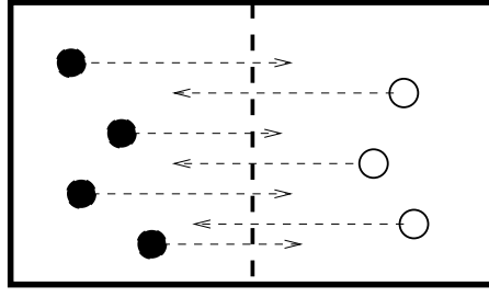
Figure 4: The Ehrenfest model (two-chambers urn).
