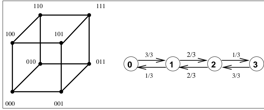
Figure 5: The complete and reduced Markov chains describing the Ehrenfest urn for N = 3 .
