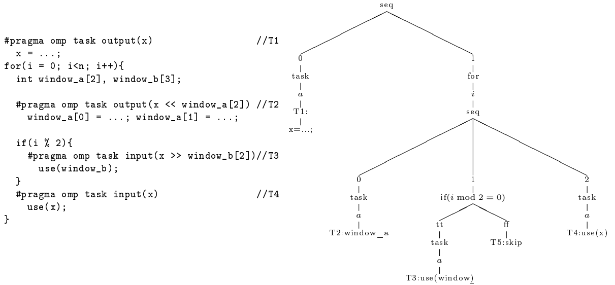
Figure 4: Program example (see Fig. 2) and corresponding AST.
