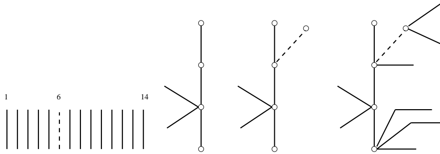
Fig. 4: Construction of trees of T_{14} with \alpha = 3 , \beta = 2 and h = 6 .
