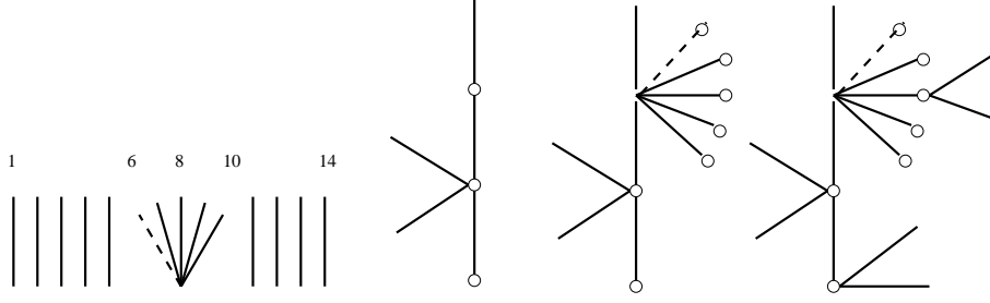
Fig. 5: Construction of trees of T_{14} with h = 6 and b - 2 = 6 .
