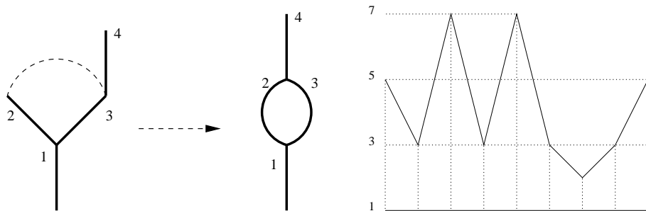
Fig. 3: Gluings of the second type and corresponding walk
