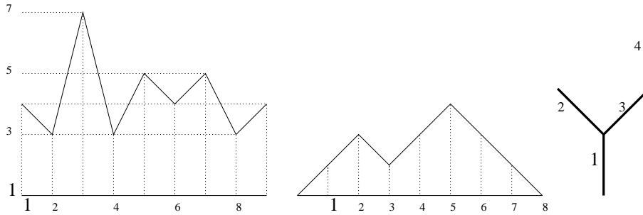
Fig. 1: Set I'_8 = (4, 3, \dots, 4) , corresponding random walk and tree \tau .
