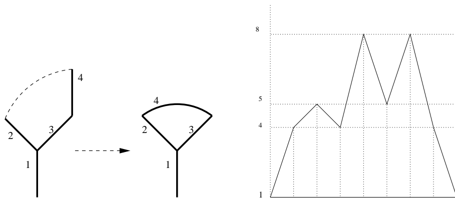
Fig. 2: Gluings of the first type and corresponding walk
