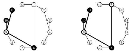
Fig. 3: Selecting the nodes \{6, 10, 11\} , we get that the ancestor-tree has size 5 and the spanning subtree has size 4.
