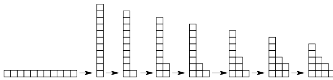
Fig. 14: Path from P = 1, 1, \dots, 1 to a partition in a circuit in \mathcal{P}(11) .
