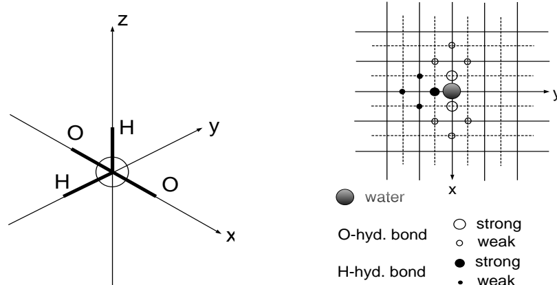
Fig. 1: The figure on the left shows the geometrical structure of the water molecules. The right figure shows a two dimensional slice of the local field configuration building up the hydrogen bonds.
