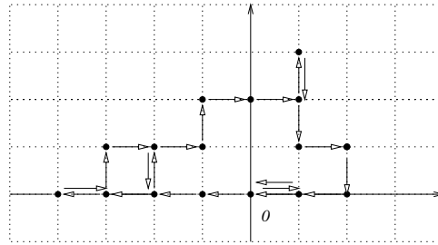
Fig. 2: A C^+ path with 22 steps.
