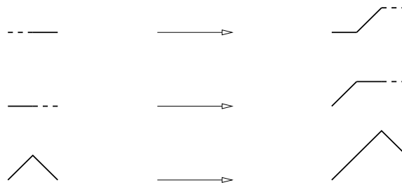
Fig. 10: The bijection between the positive cycles of length 2 and J_3 .
