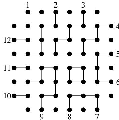
Figure 15: A fully packed loop state of order 6.
