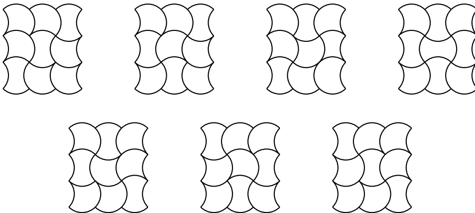
Figure 11: The seven tilings of an order-3 supergasket with gaskets and baskets.
