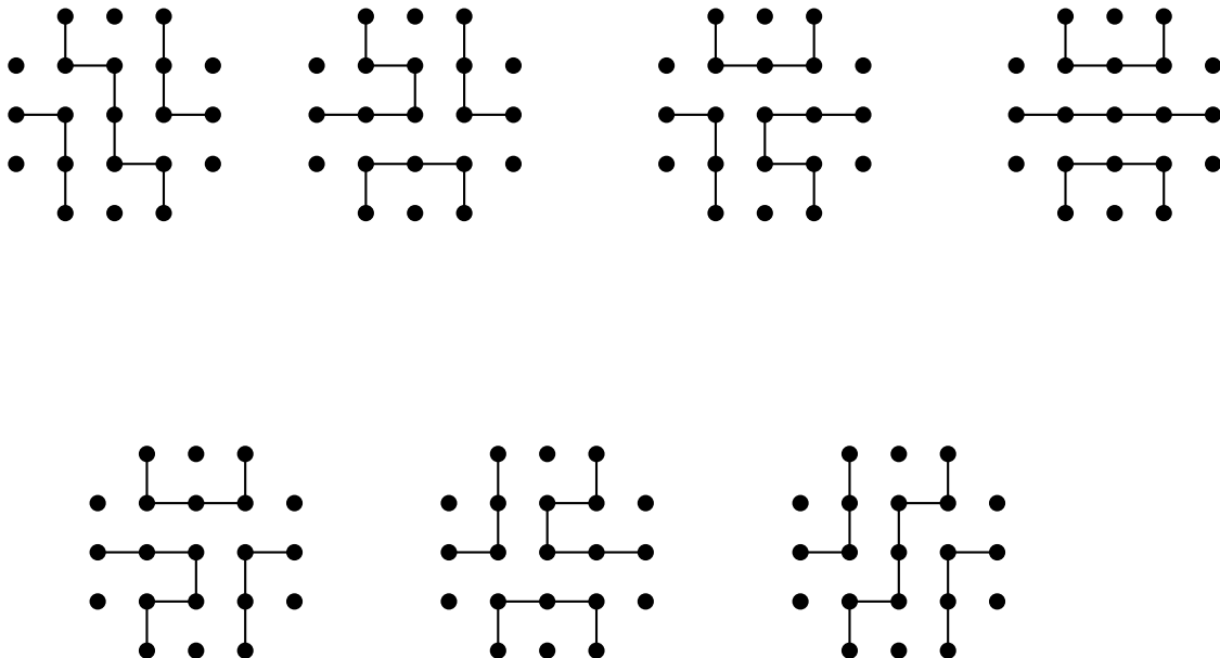
Figure 14: The seven FPL states of order 3.
