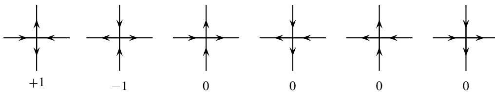
Figure 8: The six vertex-types for the square-ice model.
