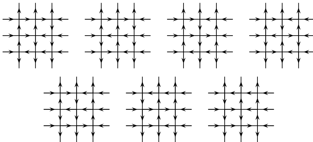
Figure 9: The seven square-ice states for n = 3 with domain-wall boundary conditions.
