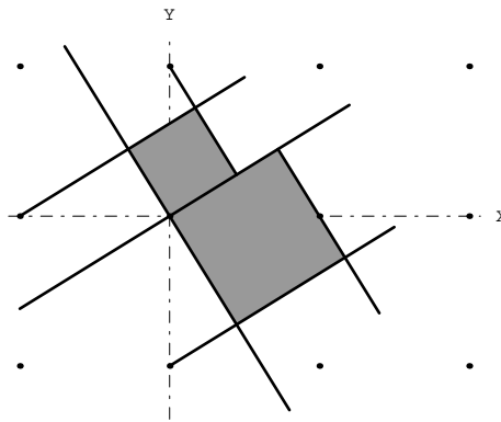
Fig. 2: The space of tilings generated by the Fibonacci tiling
