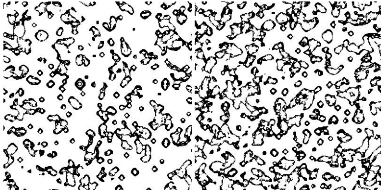
Fig. 13: The left half of the figure is time 10 of LtL rule (5,34,47,34,60) run on a 400 \times 400 lattice with periodic boundary conditions starting from product measure with density 1/2 . The right half depicts time 200.
