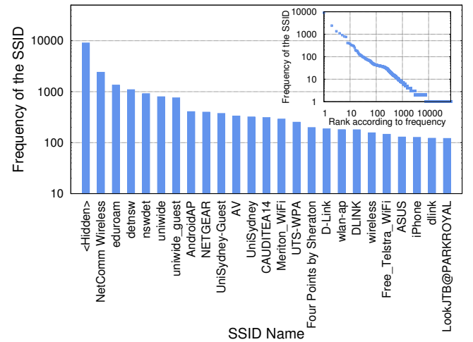
Fig. 2: SSID Popularity
