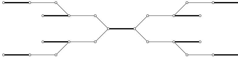
Fig. 2: A tree of the family \mathcal{T} obtained only by rule (a).
