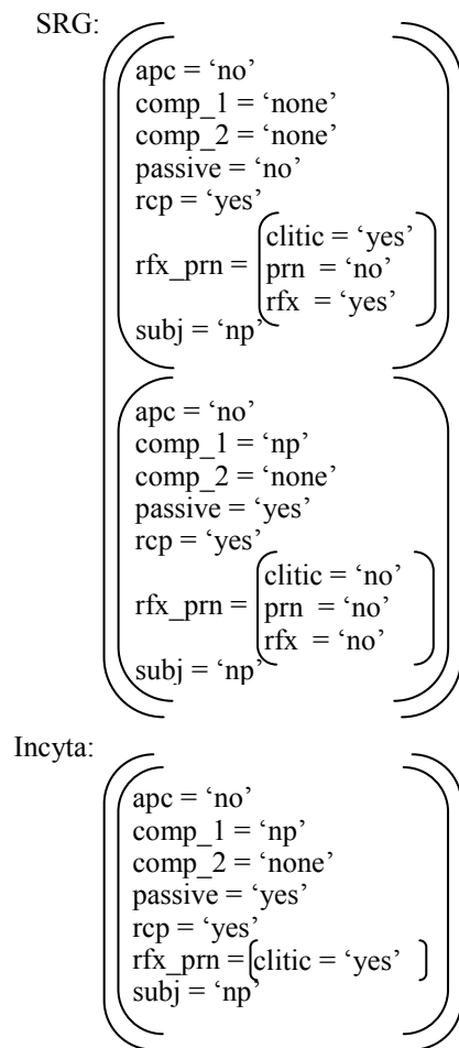
Figure 2: Example of unification problem for a reflexive verbs, such as 'cubrir' ('to cover')
