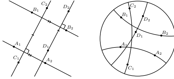
Fig. 17: The postulate of parallelism of perpendicular transversals.
