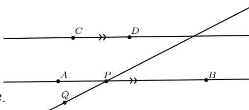
Fig. 58: Figure for proposition 11.
