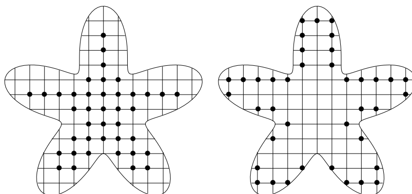
Figure 2: Left: regular nodes, i.e. belonging to \Omega_h^{**} , right: irregular nodes, i.e. belonging to \Omega_h^* .
