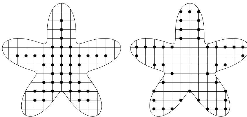
Figure 2: Left: nodes belonging to \Omega_h^{**} , right: nodes belonging to \Gamma_h^* .
