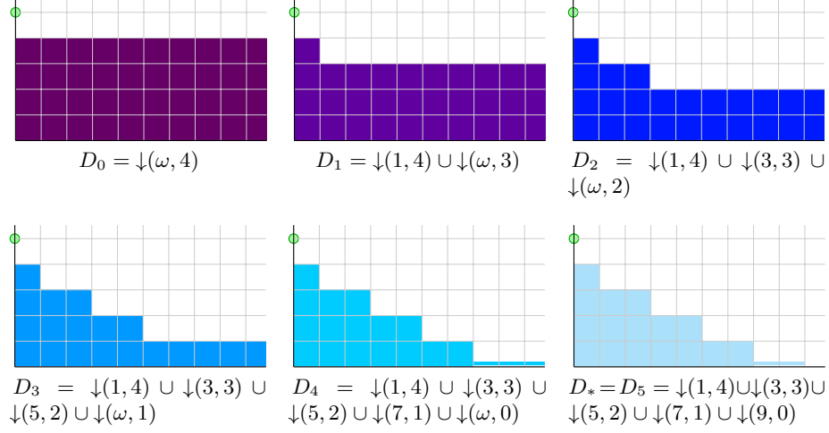
Fig. 1. The successive D_k for A_{+2} with target t = (0, 5) .
