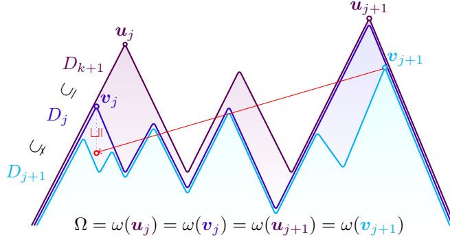
FIGURE 4. Schematic view of the proof of Claim 4.5 for j \in \{k+1, \dots, k'-1\} . The red connection witnesses \omega -monotonicity: \mathbf{v}_{j+1} \rightarrow \mathbf{v}_{j+1} + \mathbf{a} \sqsubseteq \mathbf{v}_j for some \mathbf{a} \in \mathbf{A} by Claim 4.2, and this implies \omega(\mathbf{v}_{j+1}) \subseteq \omega(\mathbf{v}_j) .
