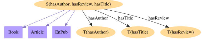
Figure 3: Baseline summary B_{G_0} for the sample graph G_0 .
