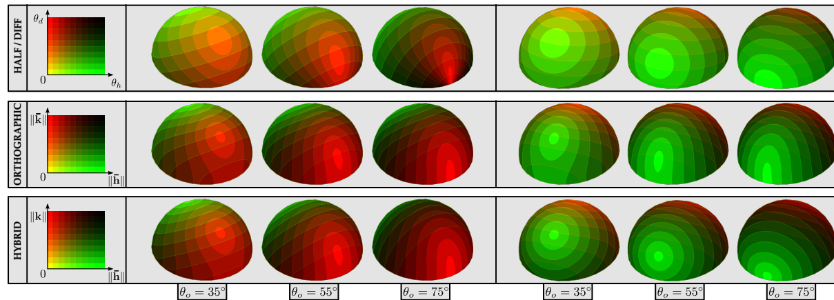
Figure 1: The three BRDF parameterizations (one per row) considered in our study. The first column shows the same color code we use for each parameterization axis. The remaining columns visualize each parameterization on a hemisphere, for three successive viewing elevations. The first set of images focus on the mirror direction, the last set on the back direction.
