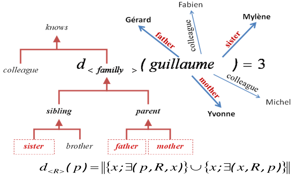
Figure 4 The simple example of a semantically parameterized degree
