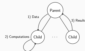
Figure 7: Code propagation
