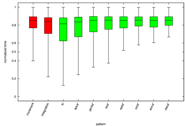
Fig. 8. Distribution of timestamps of structural commits per pattern.
