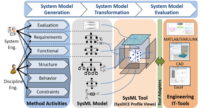
Figure 1: SysDICE overall framework
