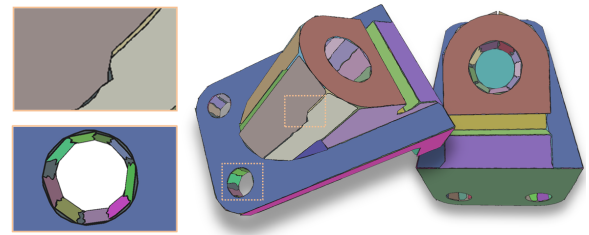
Figure 13: Detection on curved shapes. This mechanical part contains several cylindrical surface parts at different scale as well as planar parts. The regularization of planar shapes on curved surfaces may lead to the detection of irregular interfaces between shapes or over-segmentation, depicted in the lower left close-up. Some small shapes approximating the cylindrical parts are aligned to the larger planar shapes (right). Note however that the regularization of the larger planar parts is not contaminated by those cylindrical parts.
