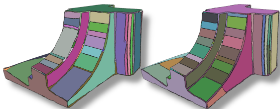
Figure 14: Stability on curved shapes. The fandisk model exhibits surface parts with different curvature. Our method approximates curved areas by smaller planar shapes of different size. A small variation of the \epsilon parameter, e.g. 0.1 (left) and 0.095 (right), might lead to larger variation in the results.
