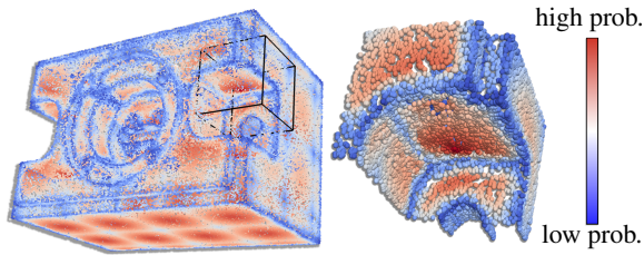
Figure 5: Seed point selection. The point set of a mechanical part is colored by the probability of a point to be chosen as a seed point for the region growing process. Points close to sharp features are assigned a low probability as their neighborhood is non-planar. On flat parts of the surface points closer to the cell center of the space decomposition are favored as they allow for a faster expansion not being bounded by the borders of the cell.
