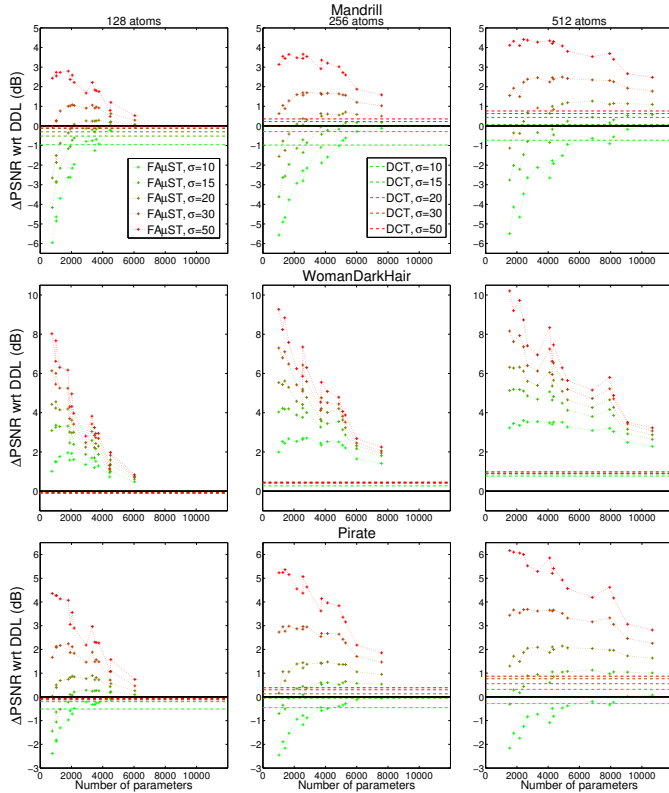
Fig. 12. Denoising results. The relative performance of FA \mu ST dictionaries compared to DDL, and the DCT compared to DDL is given for several noise levels \sigma , for various values of s_{tot} on the horizontal axis.
