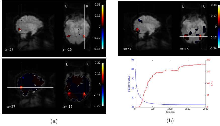
Fig. 4: (a) Output map for k=1 (TV- \ell_1 ), k=50 , and k=500 , in each case the Lateral Occipital Cortex is indicated. (b) Objective value of TV+ k -support ( k=500 ) and k-r-1 over iterations.
