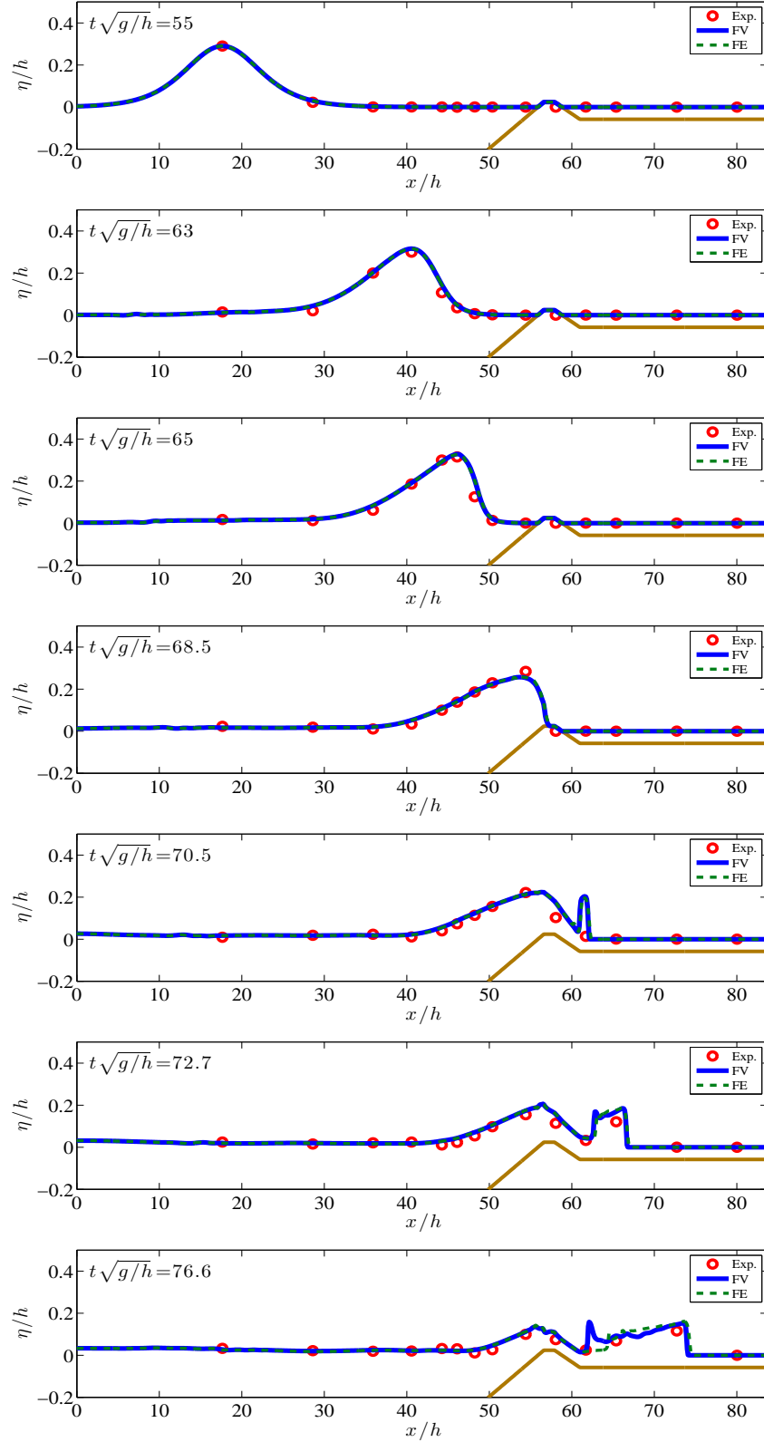
Figure 21: Evolution of surface profiles and wave transformations over an imposed reef for A/h = 0.3 and 1/12 slope
