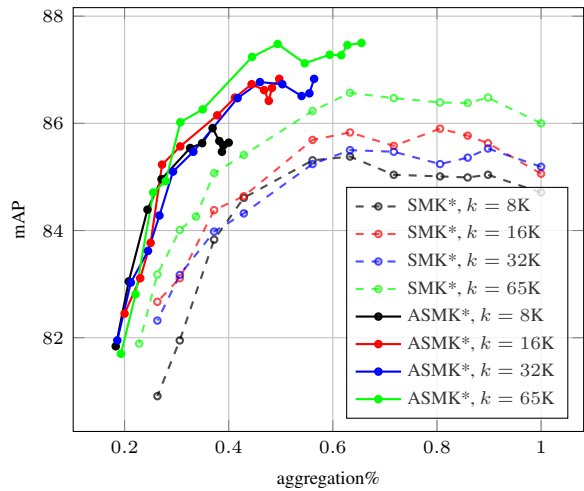
Figure 10. SMK*/ASMK* performance vs. aggregation% on Holidays-L for different vocabulary sizes k . Selectivity exponent \alpha = 3 . Asymmetric aggregation.
