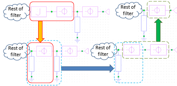
Fig. 8: Circuitual transformation to embed a constant chain matrix into a filter's output coupling; M_{N,L} is implemented by the J -inverter whereas phase shifters by -\phi blocks.
