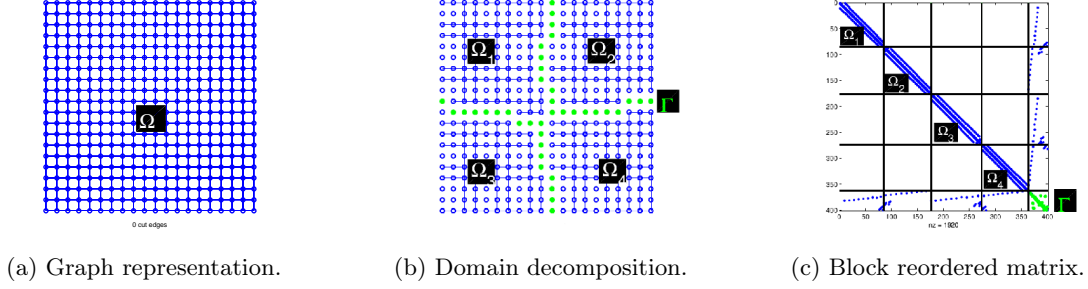
Figure 1: Domain decomposition into four subdomains \Omega_1, \dots, \Omega_4 . The initial domain \Omega may be algebraically represented with the graph G associated with the sparsity pattern of matrix \mathcal{A} (a).
