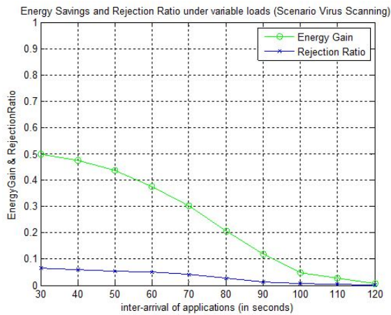
Fig. 4. Virus Scanning.
