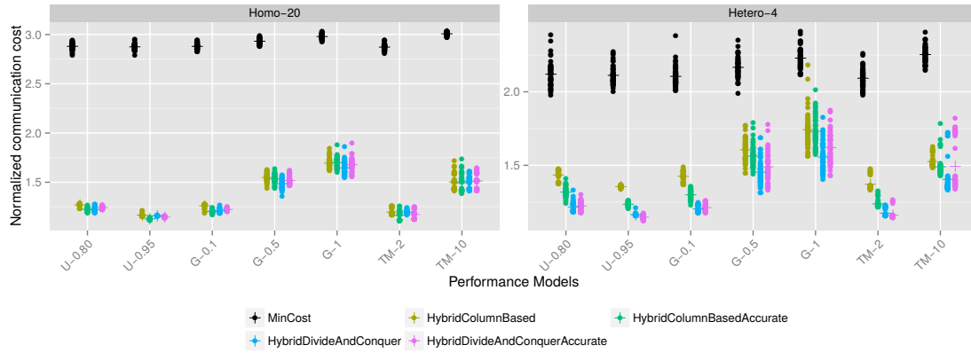
Figure 7. Communication cost of MINCOST and hybrid strategies for HOMOGENEOUS-20-CPU and HETEROGENEOUS-4-GPU for dynamic setting.
