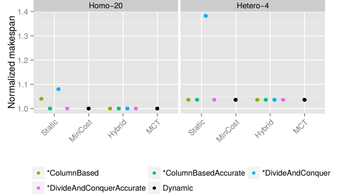
Figure 4. Makespan as a function of the chosen algorithm for HOMOGENEOUS-20-CPU and HETEROGENEOUS-4-GPU for static setting.
