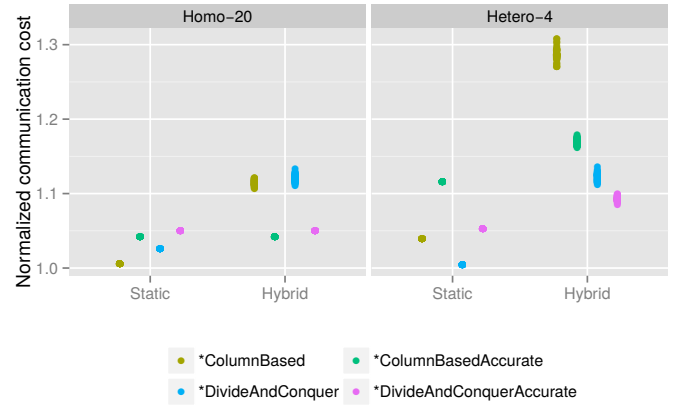
Figure 5. Communication cost of MINCOST and hybrid strategies for HOMOGENEOUS-20-CPU and HETEROGENEOUS-4-GPU for static setting
