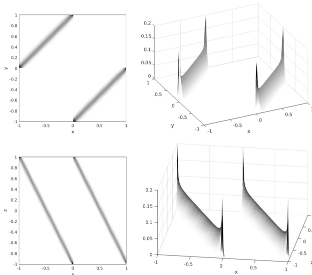
FIGURE 6. Top-Left: support of the optimal coupling \tilde{\gamma}_{12}(x,y) . Top-Right: optimal coupling \tilde{\gamma}_{12}(x,y) . Bottom-Left: support of the optimal coupling \tilde{\gamma}_{13}(x,z) . Bottom-Right: optimal coupling \tilde{\gamma}_{13}(x,z) .
