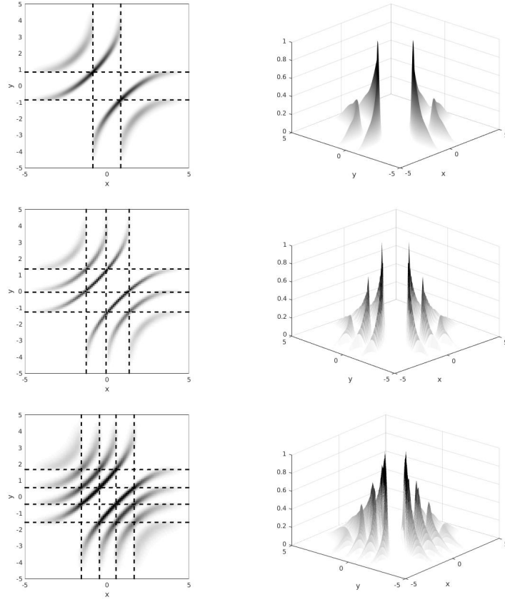
FIGURE 3. On the Left: support of the optimal coupling \hat{\gamma}_{12}(x, y) , on the Right: graph of the optimal coupling \hat{\gamma}_{12}(x, y) , in the cases N = 3 (1st Row), N = 4 (2nd Row), N = 5 (3rd Row). The dashed lines delimit the supports of \tilde{\mu}_i , with i = 1, \dots, N .
