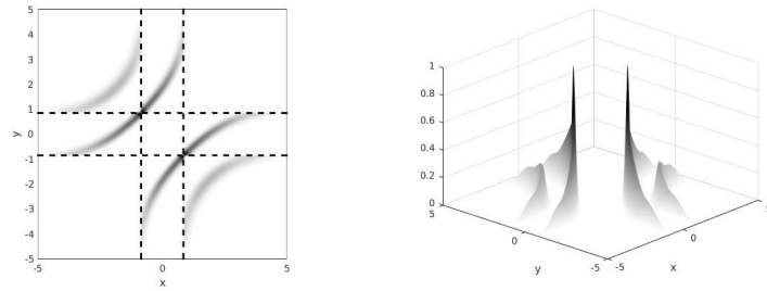
FIGURE 4. (logarithmic cost) Left: support of the optimal coupling \hat{\gamma}_{12}(x, y) for N = 3 . Right: support of the optimal coupling \hat{\gamma}_{12}(x, y) for N = 3 . The dashed lines delimit the intervals where \tilde{\mu}_i , with i = 1, \dots, 3 , are defined.
